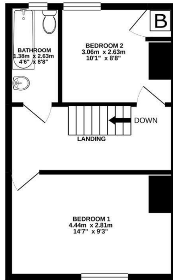
1ST FLOOR 31.0 sq.m. (334 sq.ft.) approx.
