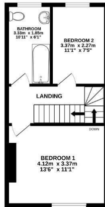
1ST FLOOR 33.8 sqm. (363 sq.ft.) approx.
