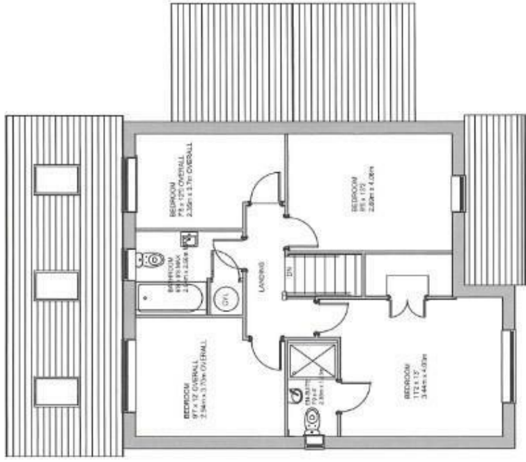
1ST FLOOR APPROX. FLOOR AREA 645 SQ.FT. (60 SQ.M)
