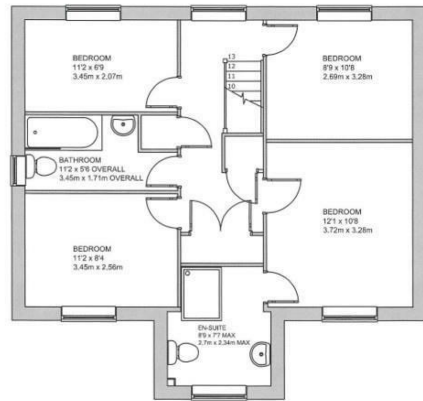
1ST FLOOR APPROX. FLOOR AREA 625 SQ.FT. (58 SQ.M)
