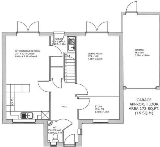
GROUND FLOOR APPROX. FLOOR (EXCLUDING GARAGE) AREA 656 SQ.FT. (62 SQ.M)
