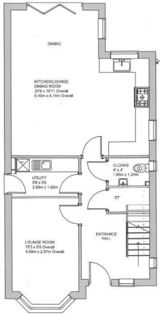
GROUND FLOOR APPROX. FLOOR AREA 764 SQ.FT. (71 SQ.M)
